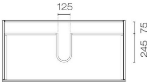
Drawer Cutout Detail
