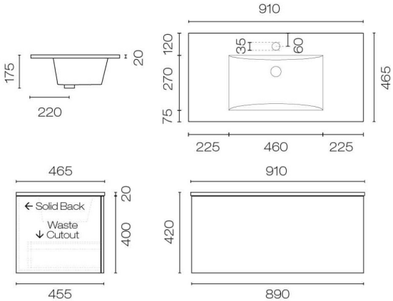
Drawer Cutout Detail
